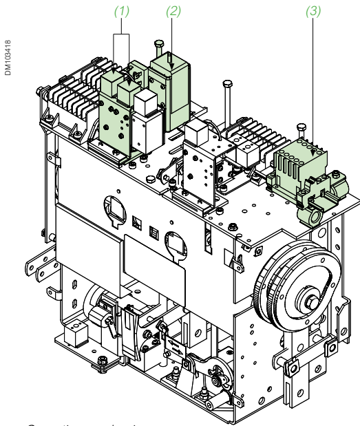
Operating mechanism
