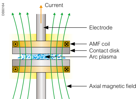
Fig. 2: cross-section of AMF contact
