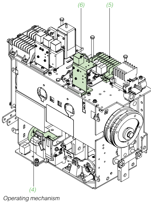
Operating mechanism (4)
