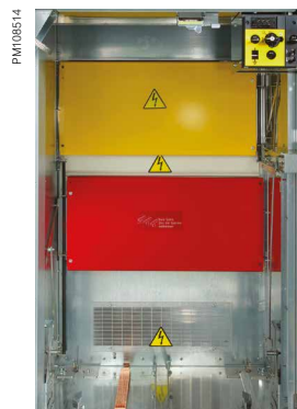
Circuit-breaker compartment
