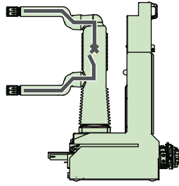
Vacuum circuit-breaker
