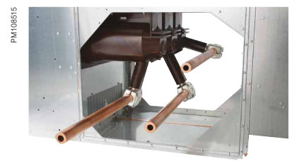
Busbar compartment
