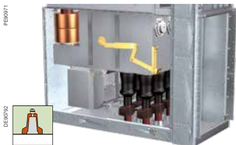
Inner cone-type bushings up to 40.5 kV - 2x size 2 (800 A) or size 3 (1250 A) with flange-mounted voltage transformers
