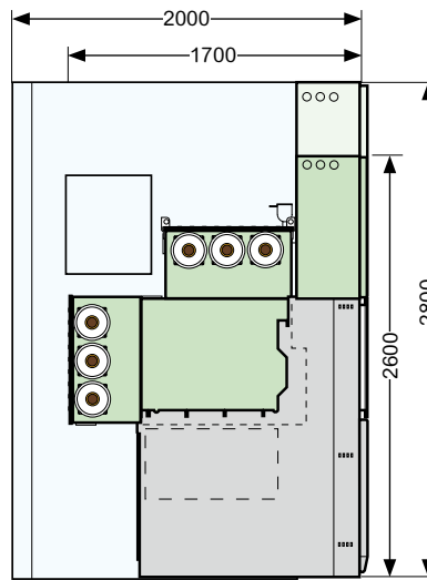
Side view - dimensions
