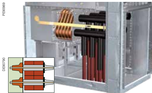
Outer cone-type bushings up to 36 kV, > 1250 A (2 outer cone-type/conductor)
