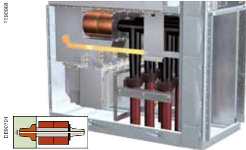
Outer cone-type bushings up to 36 kV, < 1250 A (1 outer cone-type/conductor)
